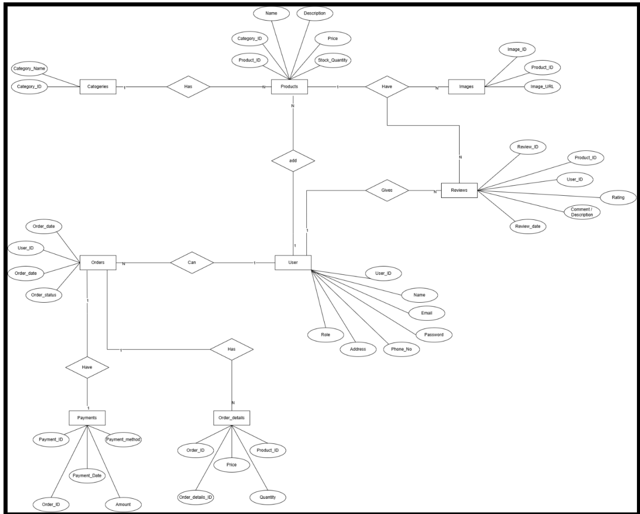
Figure 12 ERD
