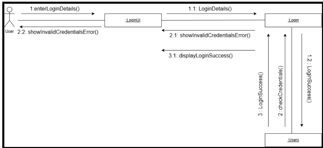
Figure 14 Collaboration Diagram
